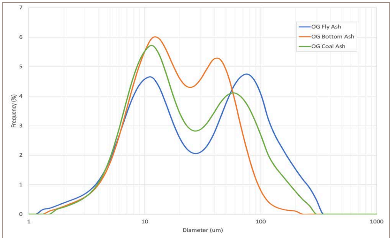
Example Particle Size Distribution – Oak Grove Fly Ash and Milled Bottom Ash*
